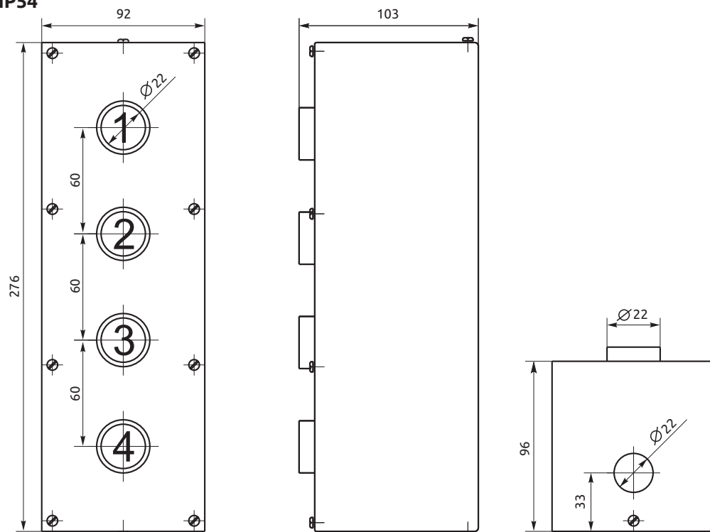
Metal push-button box BoxM1-4 IP40 BoxM2-4 IP54
