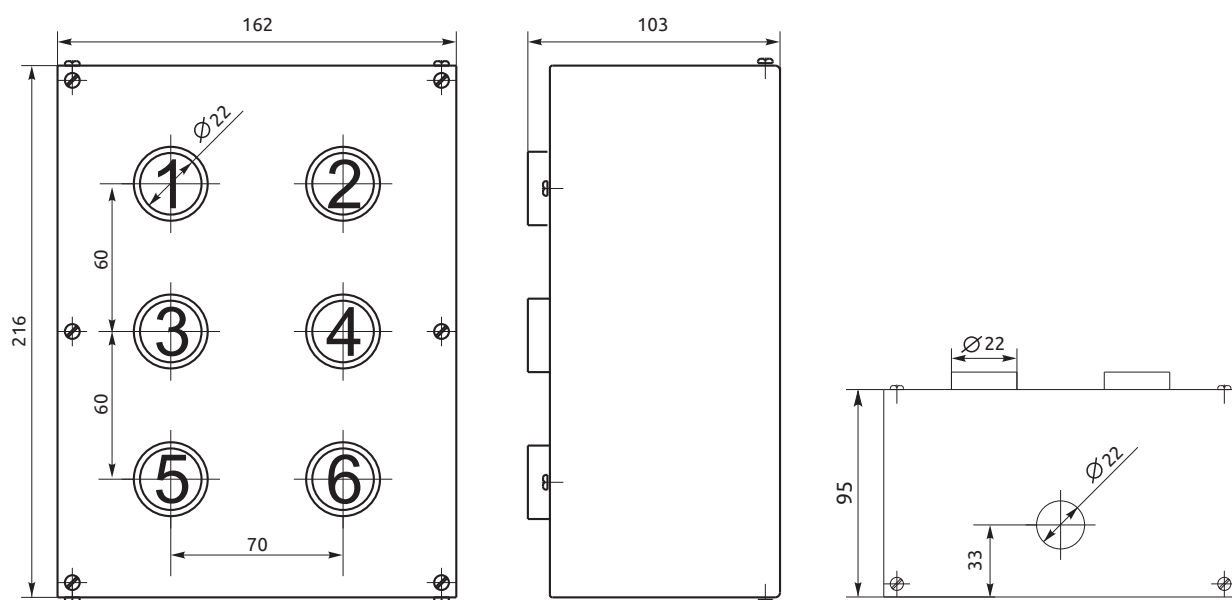
Metal push-button box BoxM1-6 IP40 BoxM2-6 IP54
