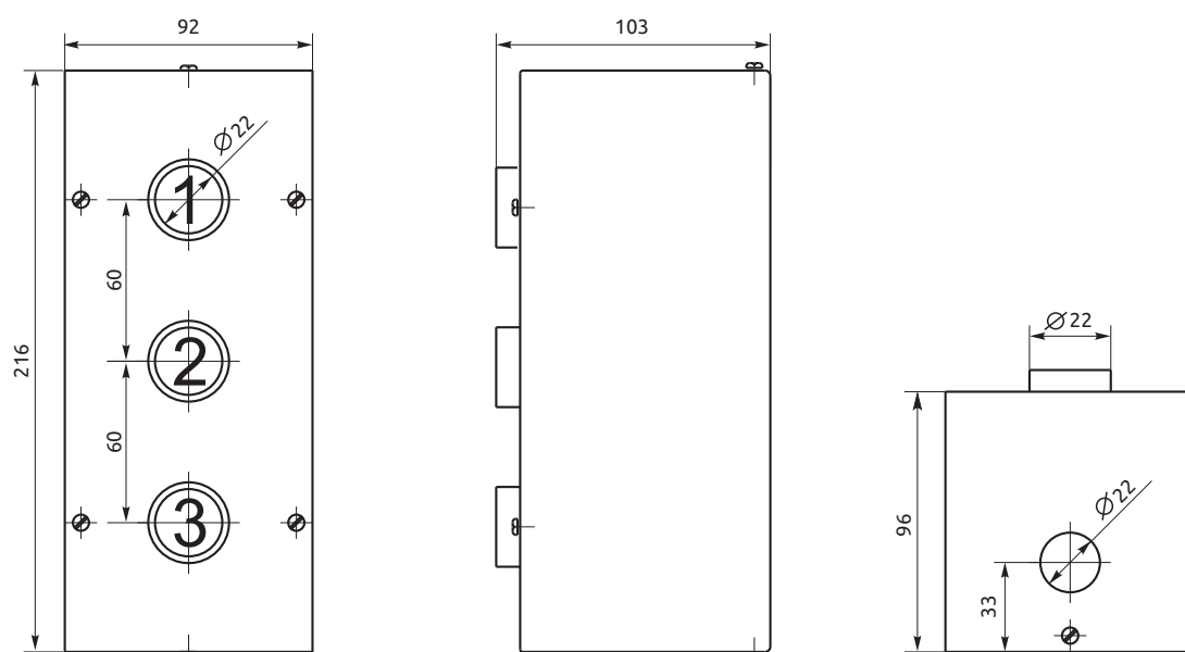
Metal push-button box BoxM1-3 IP40 BoxM2-3 IP54
