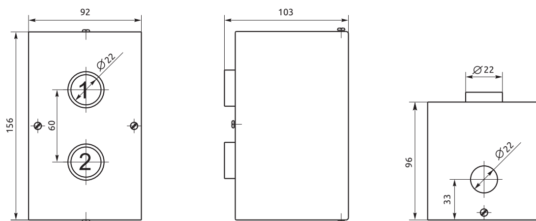
Metal push-button box BoxM1-2 IP40 BoxM2-2 IP54
