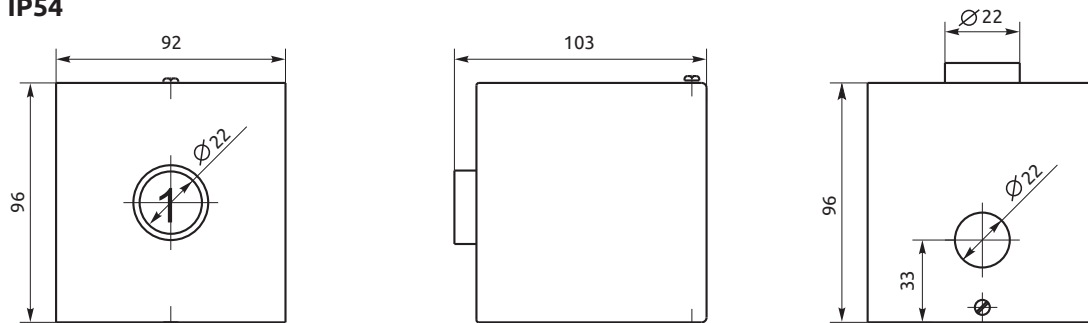
Metal push-button box BoxM1-2 IP40 BoxM2-2 IP54
